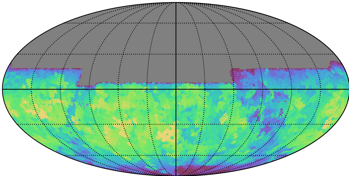
baseline_v2.1_10yrs All sky y band: Max saturation_mag
