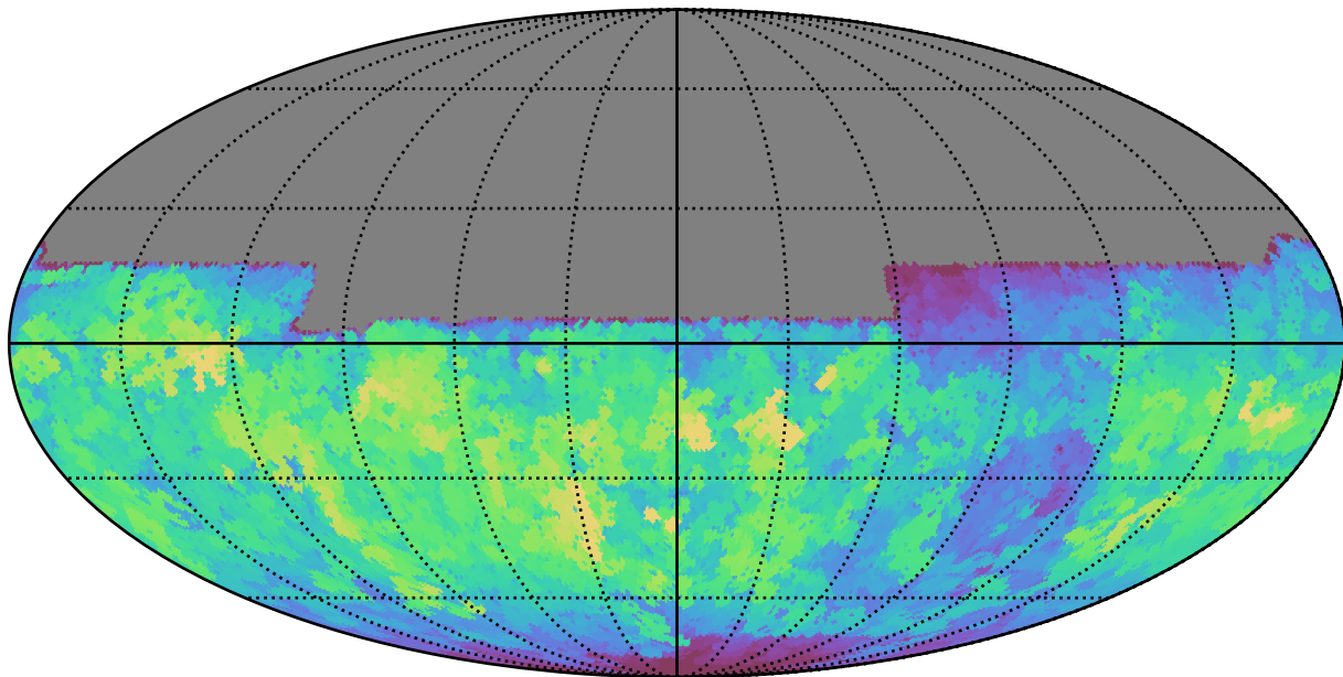
baseline_v2.1_10yrs All sky u band: Max saturation_mag
