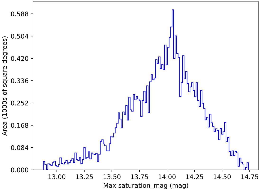
baseline_v2.1_10yrs All sky u band: Max saturation_mag
