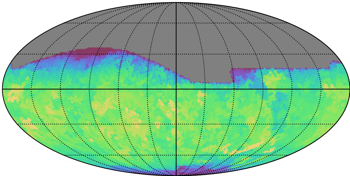
baseline_v2.1_10yrs All sky r band: Max saturation_mag
