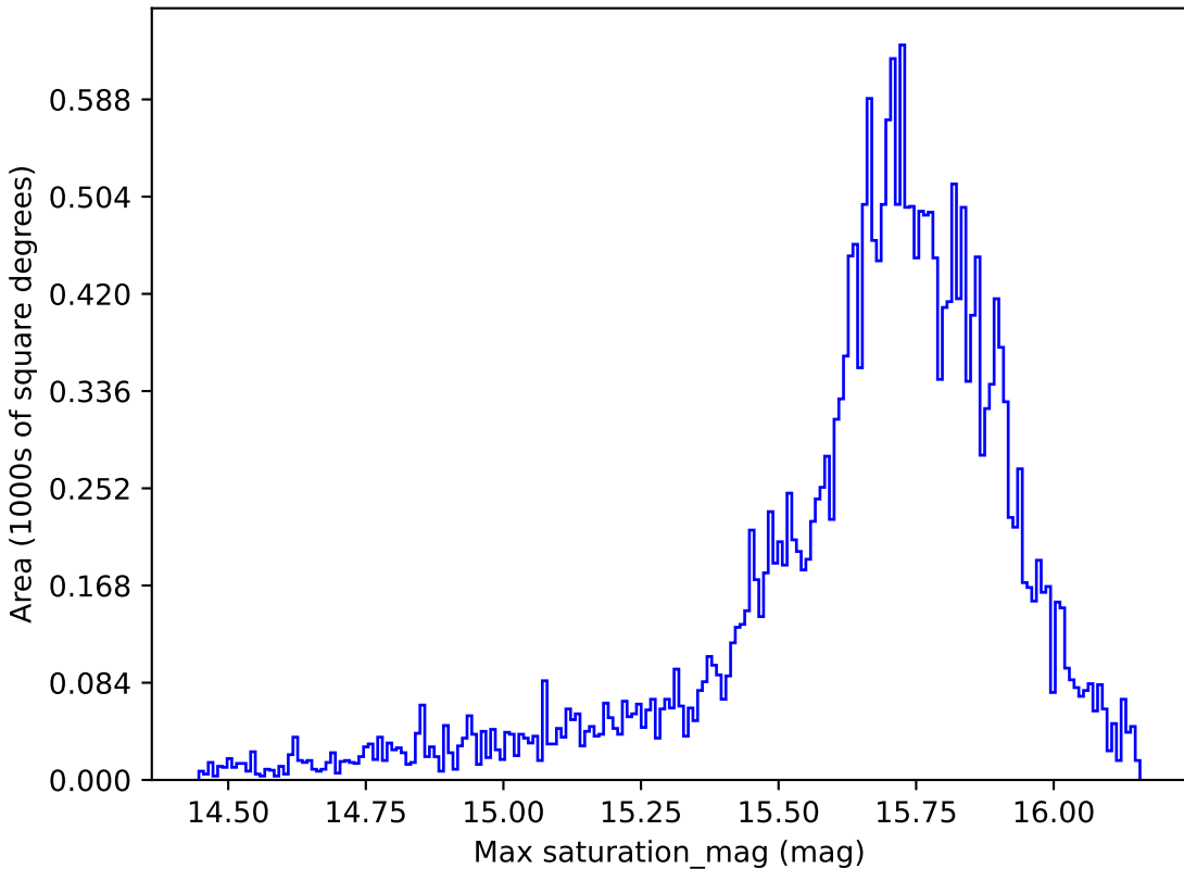
baseline_v2.1_10yrs All sky r band: Max saturation_mag
