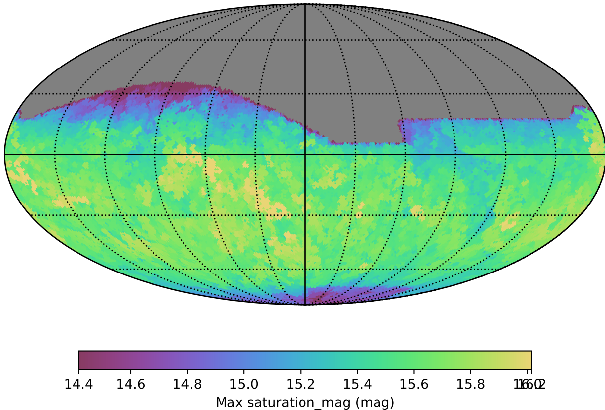
baseline_v2.1_10yrs All sky i band: Max saturation_mag
