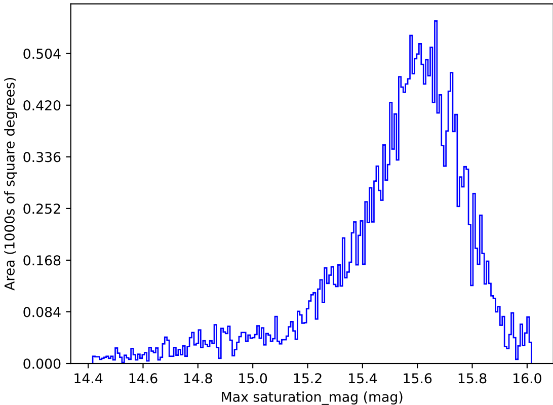
baseline_v2.1_10yrs All sky i band: Max saturation_mag
