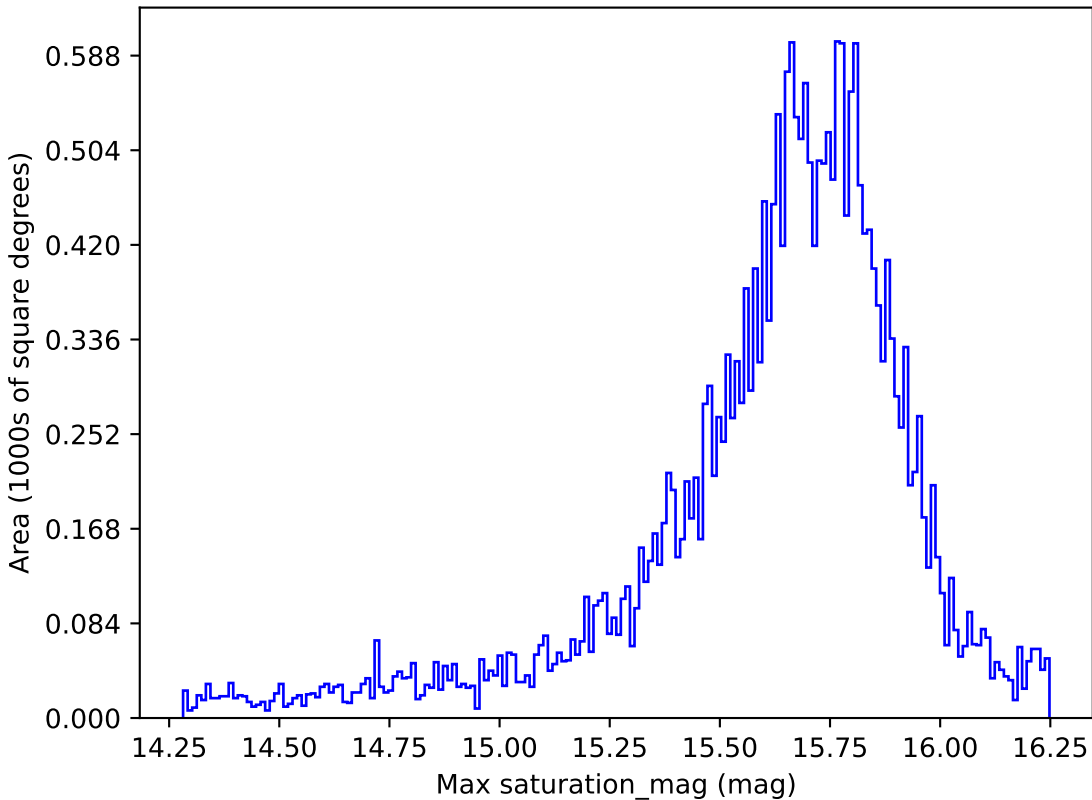
baseline_v2.1_10yrs All sky g band: Max saturation_mag
