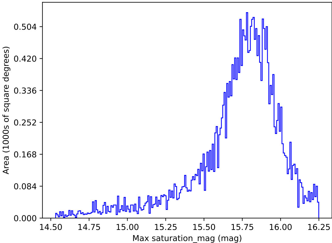
baseline_v2.1_10yrs All sky all bands: Max saturation_mag
