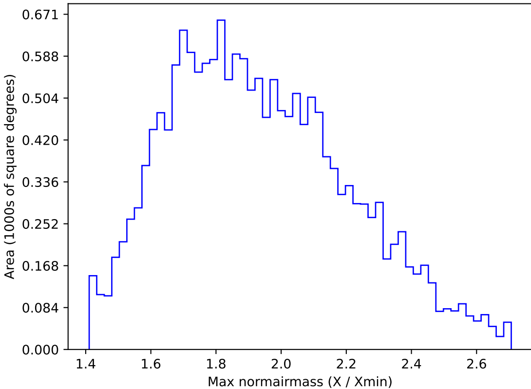
baseline_v2.1_10yrs WFD z band: Max normairmass
