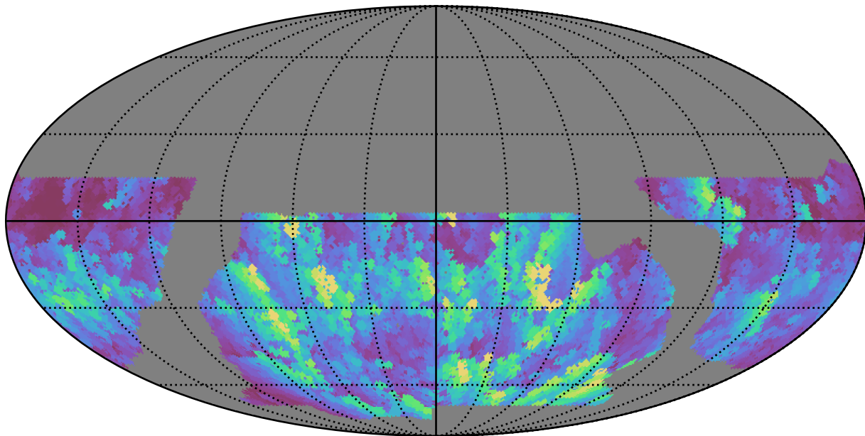
baseline_v2.1_10yrs WFD u band: Max normairmass
