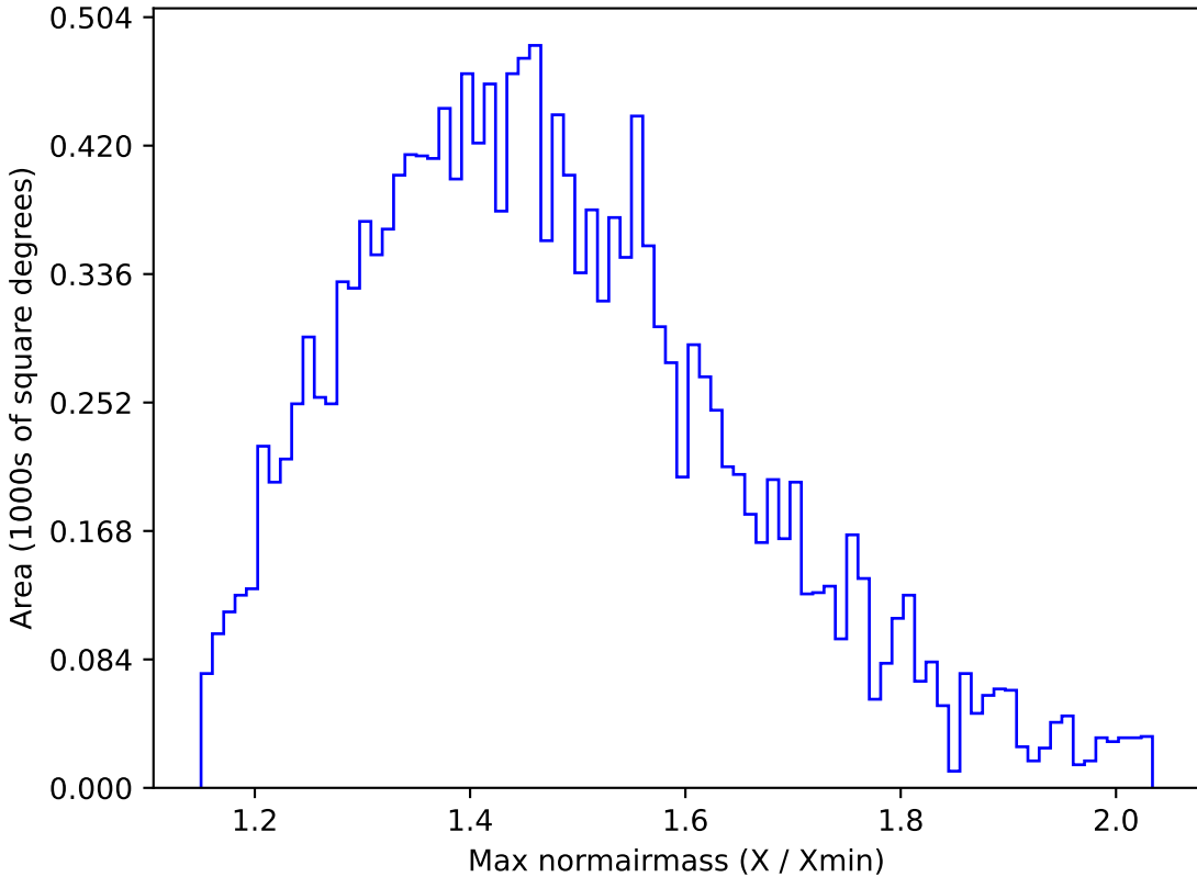
baseline_v2.1_10yrs WFD u band: Max normairmass
