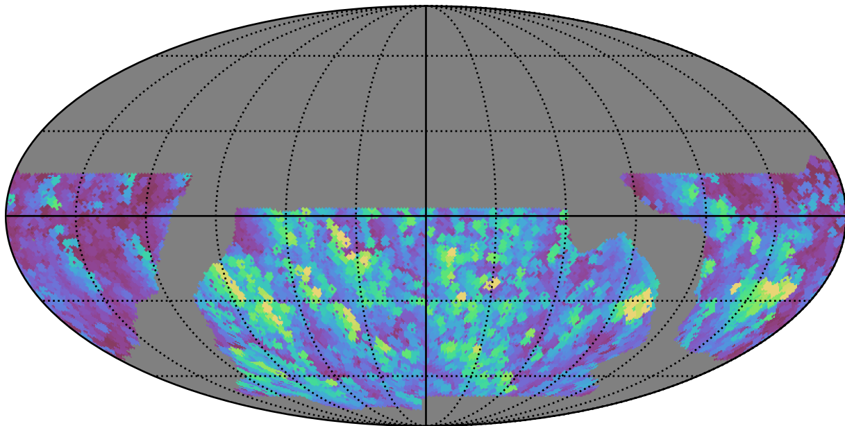
baseline_v2.1_10yrs WFD r band: Max normairmass
