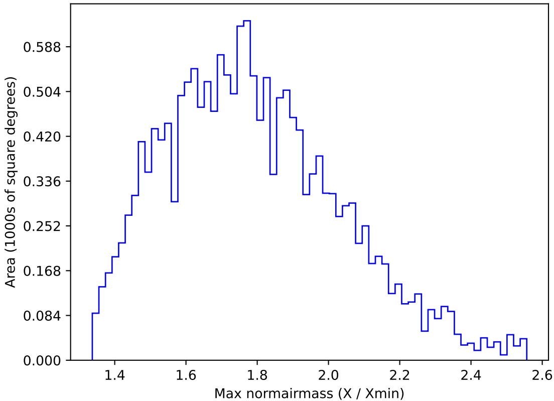
baseline_v2.1_10yrs WFD r band: Max normairmass
