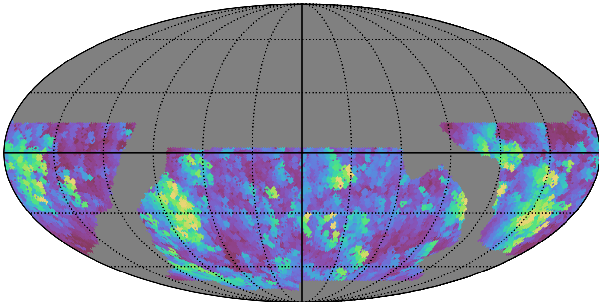
baseline_v2.1_10yrs WFD i band: Max normairmass
