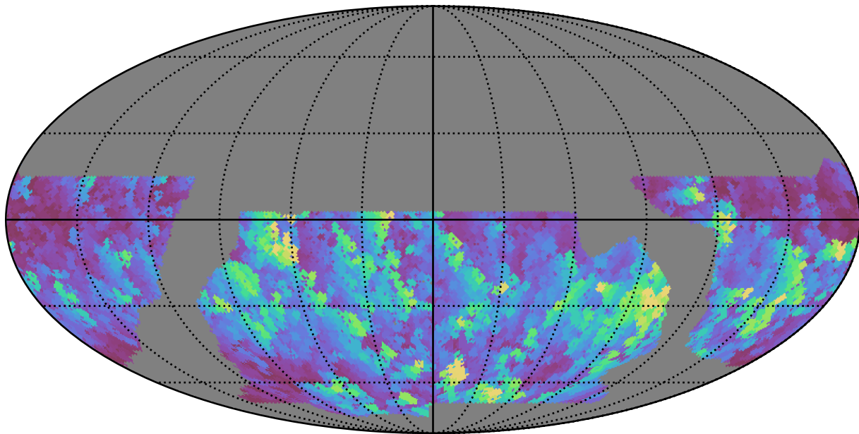
baseline_v2.1_10yrs WFD g band: Max normairmass
