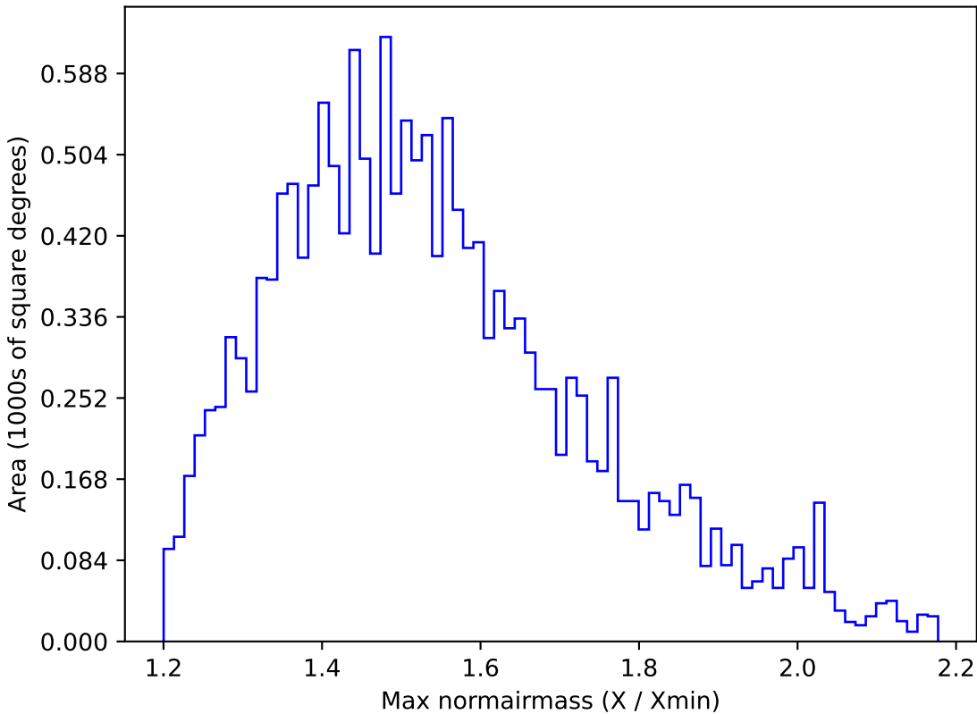
baseline_v2.1_10yrs WFD g band: Max normairmass
