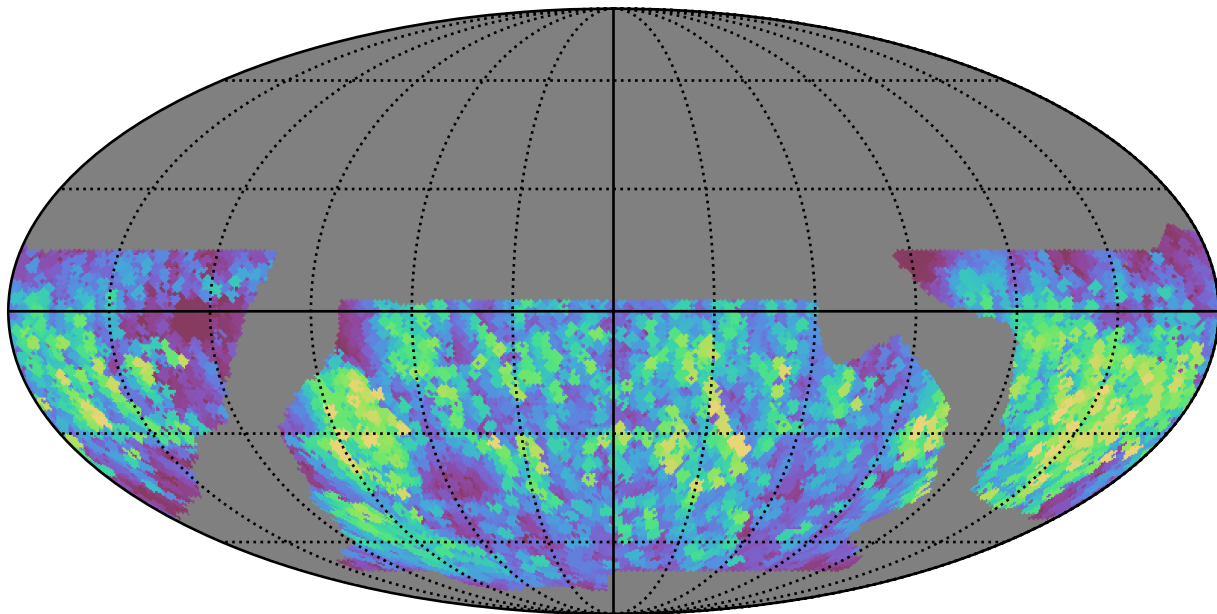
baseline_v2.1_10yrs WFD all bands: Max normairmass
