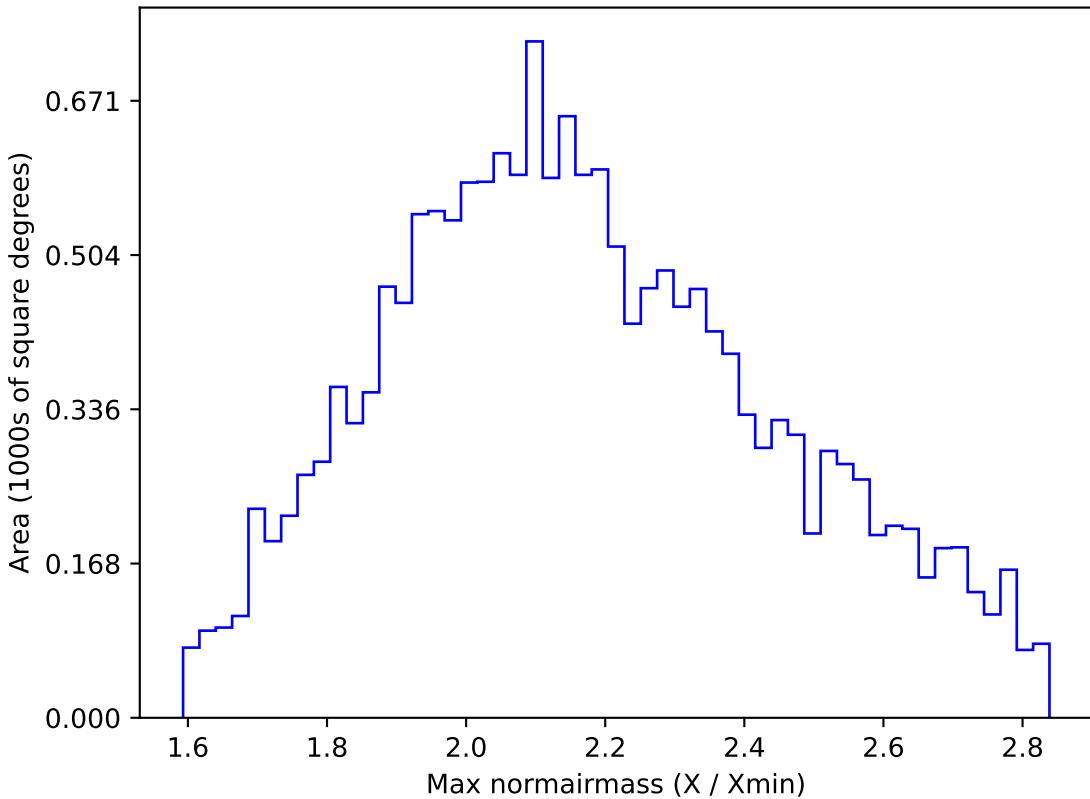
baseline_v2.1_10yrs WFD all bands: Max normairmass
