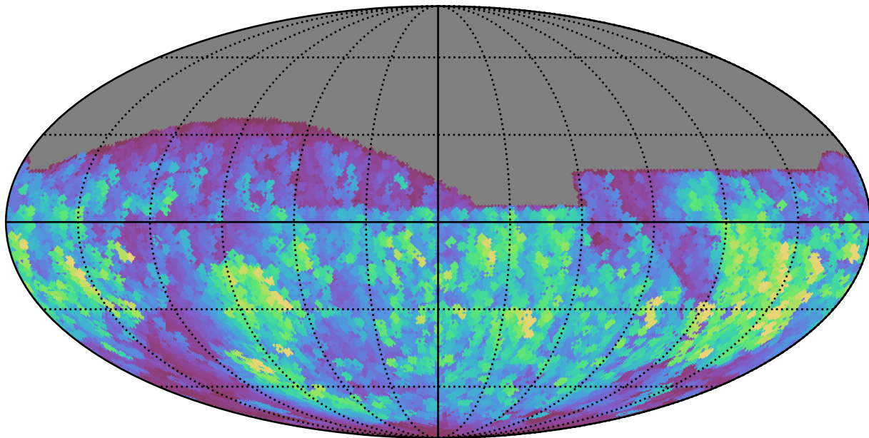
baseline_v2.1_10yrs All sky z band: Max normairmass
