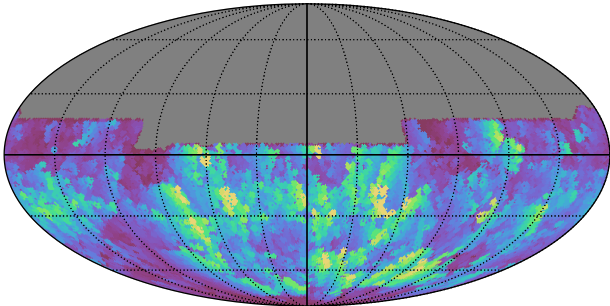
baseline_v2.1_10yrs All sky u band: Max normairmass
