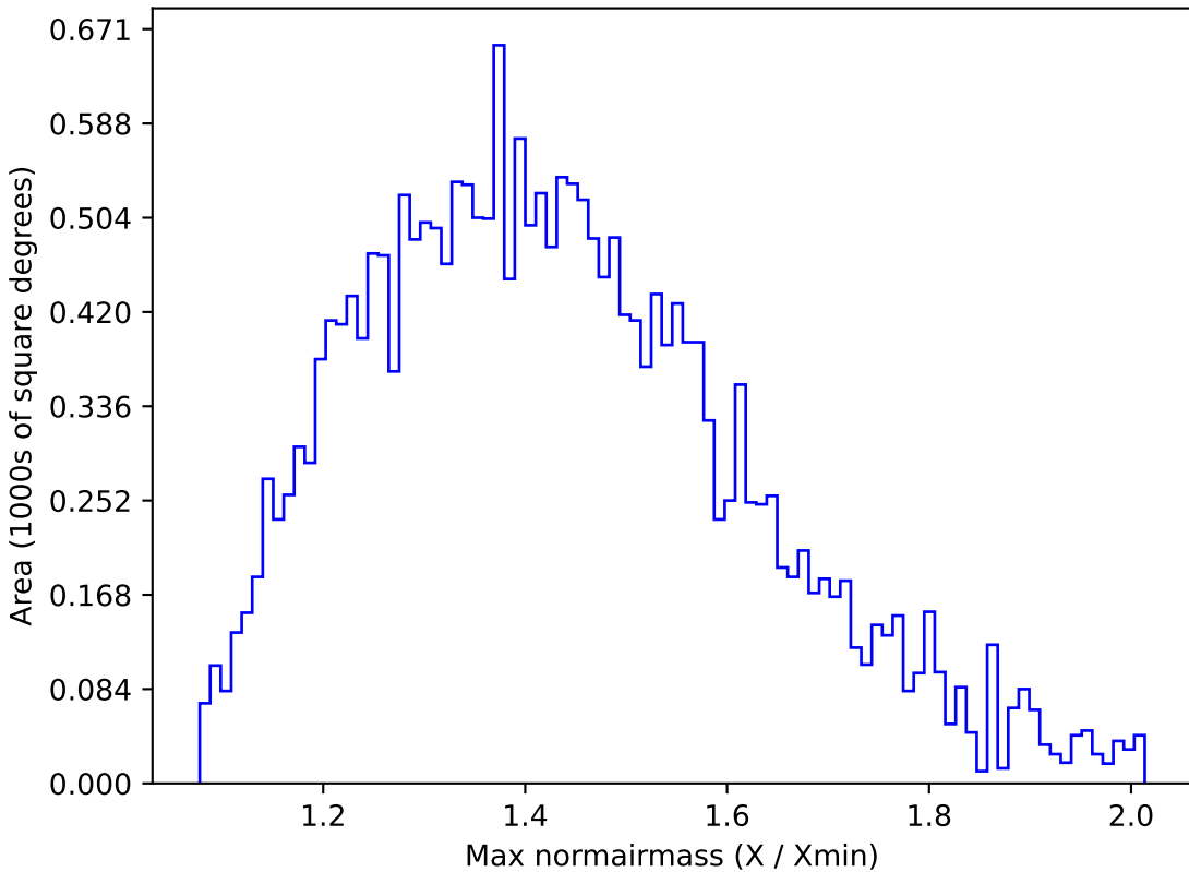
baseline_v2.1_10yrs All sky u band: Max normairmass
