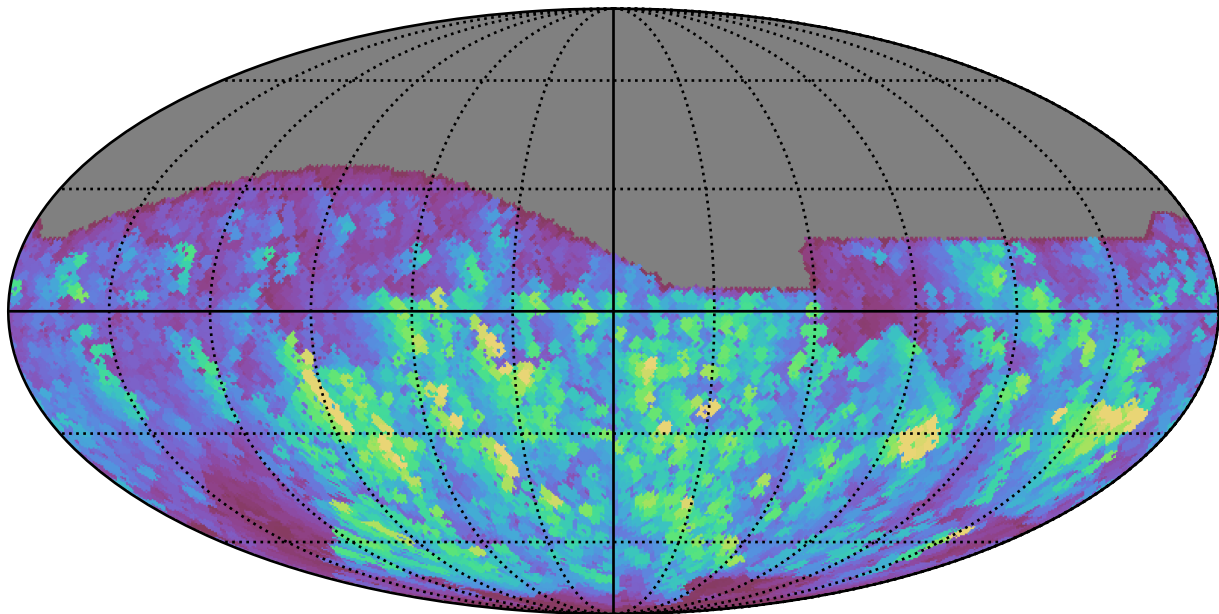
baseline_v2.1_10yrs All sky r band: Max normairmass
