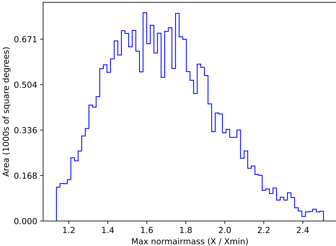
baseline_v2.1_10yrs All sky r band: Max normairmass
