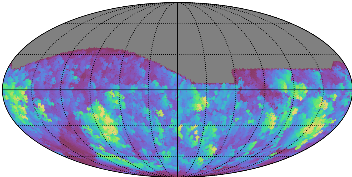
baseline_v2.1_10yrs All sky i band: Max normairmass
