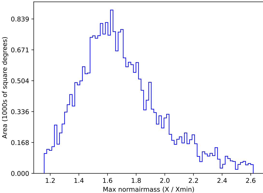
baseline_v2.1_10yrs All sky i band: Max normairmass
