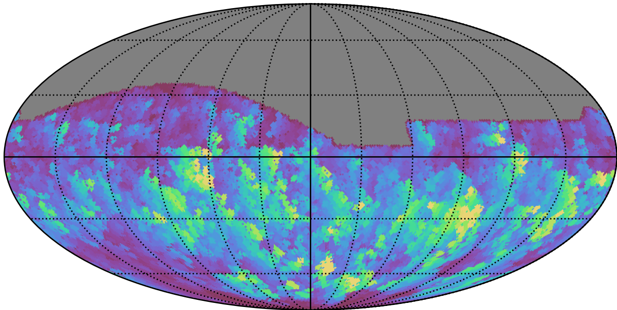
baseline_v2.1_10yrs All sky g band: Max normairmass
