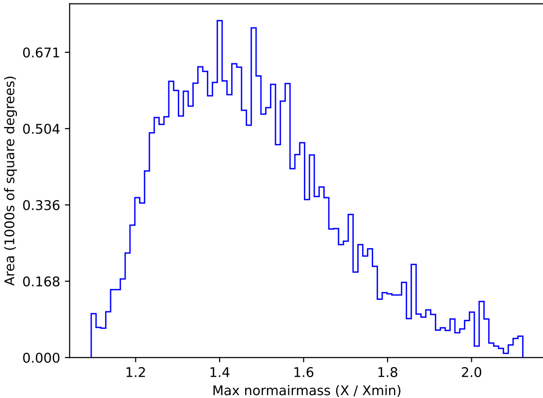
baseline_v2.1_10yrs All sky g band: Max normairmass
