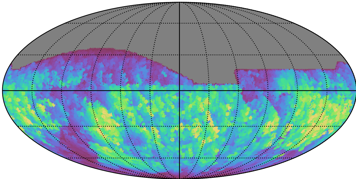
baseline_v2.1_10yrs All sky all bands: Max normairmass
