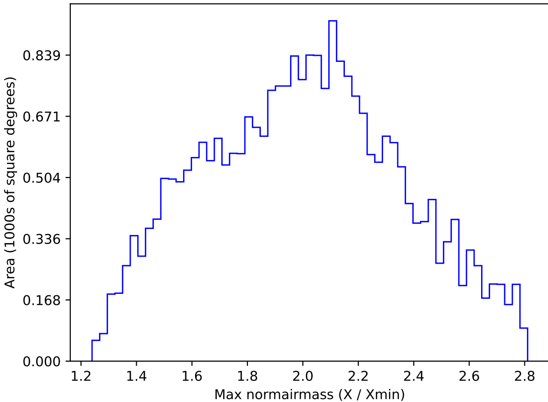
baseline_v2.1_10yrs All sky all bands: Max normairmass
