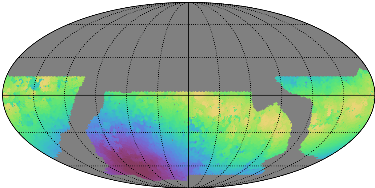
baseline_v2.1_10yrs WFD z band: Max moonDistance
