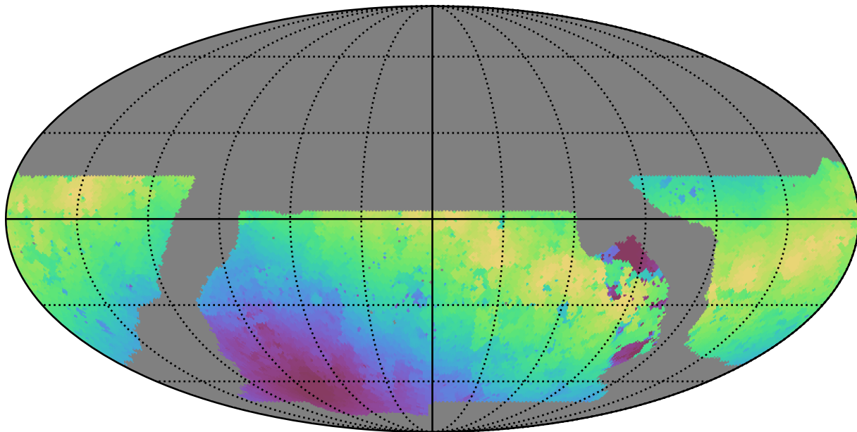
baseline_v2.1_10yrs WFD y band: Max moonDistance
