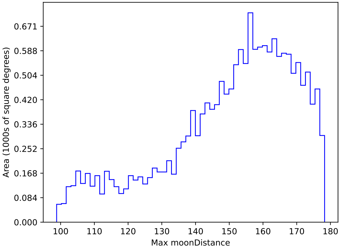
baseline_v2.1_10yrs WFD y band: Max moonDistance
