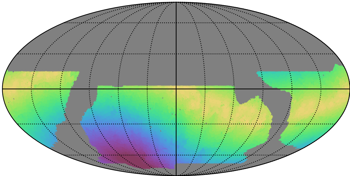
baseline_v2.1_10yrs WFD u band: Max moonDistance
