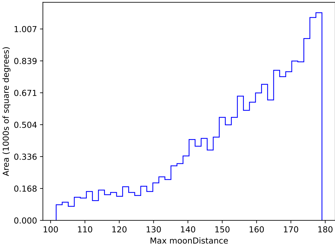
baseline_v2.1_10yrs WFD u band: Max moonDistance
