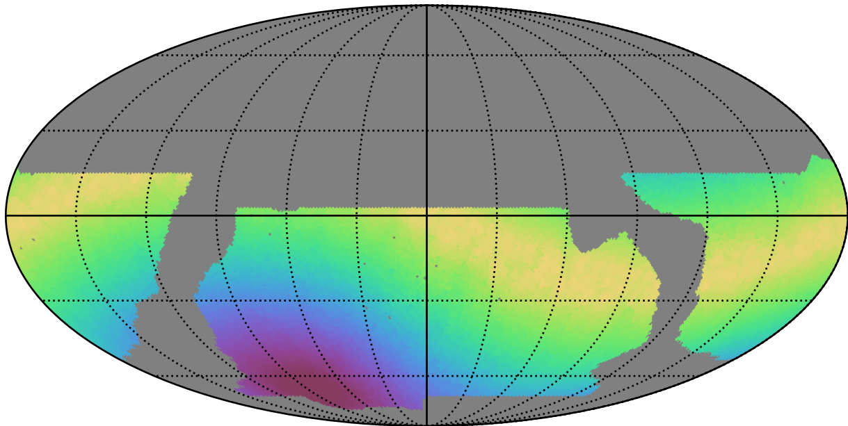
baseline_v2.1_10yrs WFD r band: Max moonDistance
