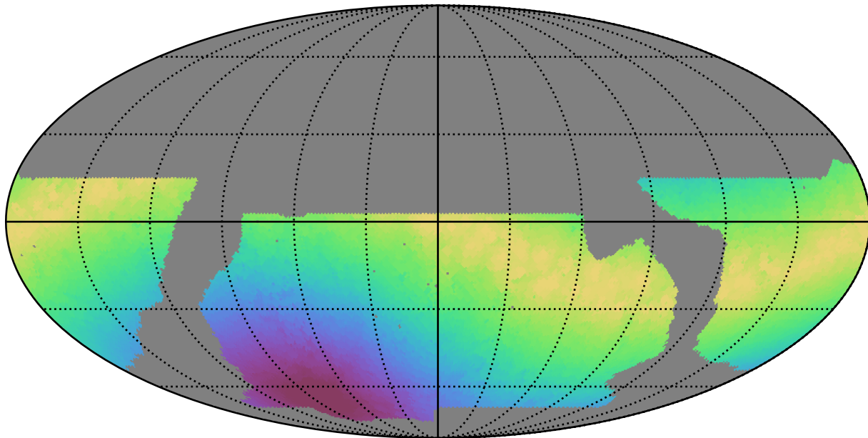
baseline_v2.1_10yrs WFD i band: Max moonDistance
