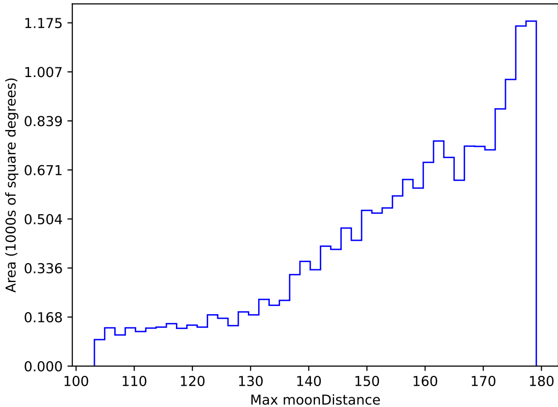
baseline_v2.1_10yrs WFD i band: Max moonDistance
