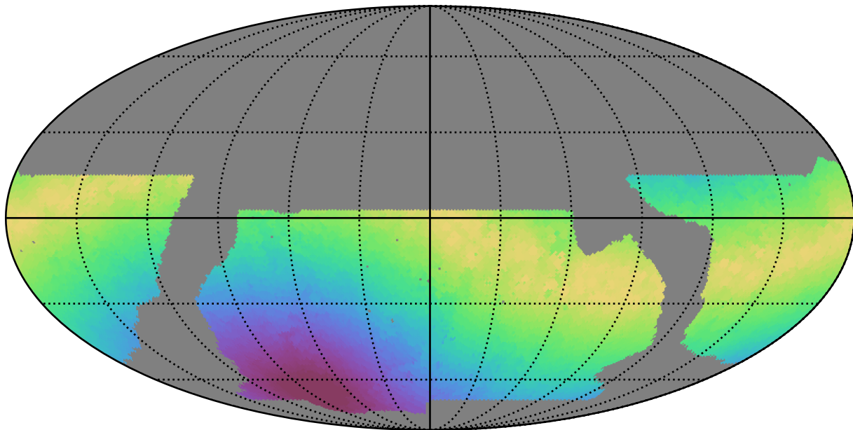
baseline_v2.1_10yrs WFD g band: Max moonDistance
