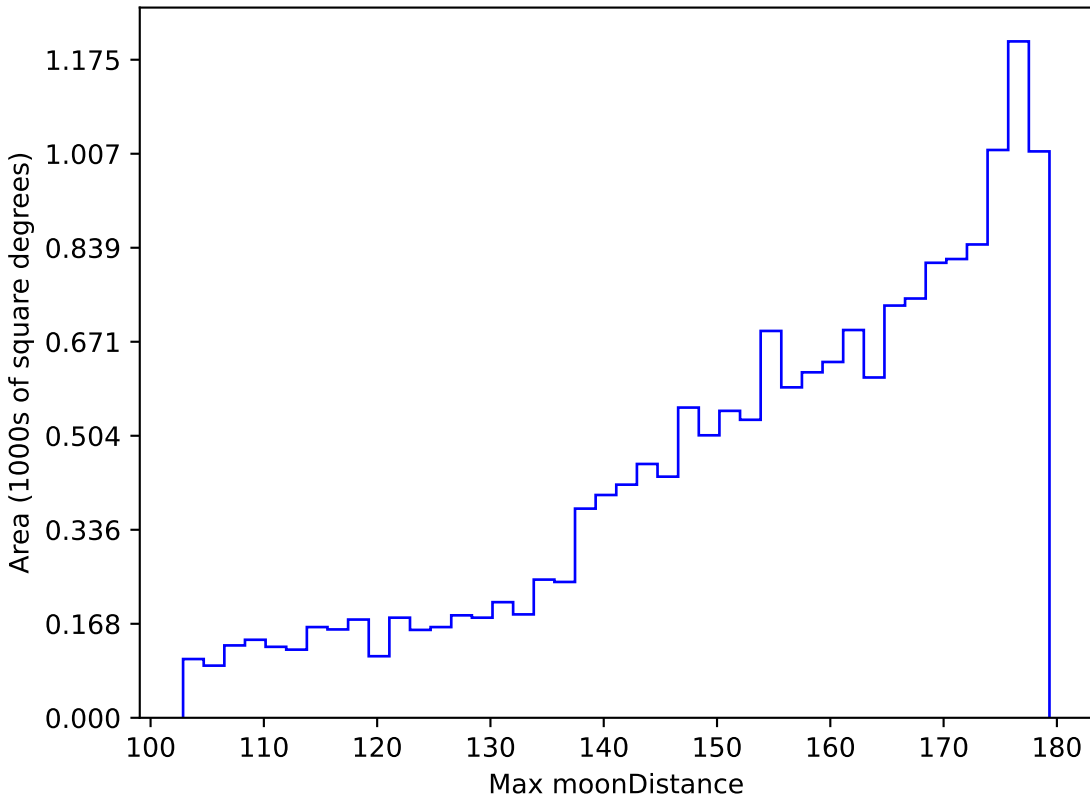
baseline_v2.1_10yrs WFD g band: Max moonDistance
