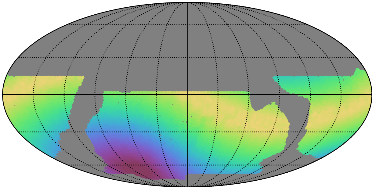
baseline_v2.1_10yrs WFD all bands: Max moonDistance
