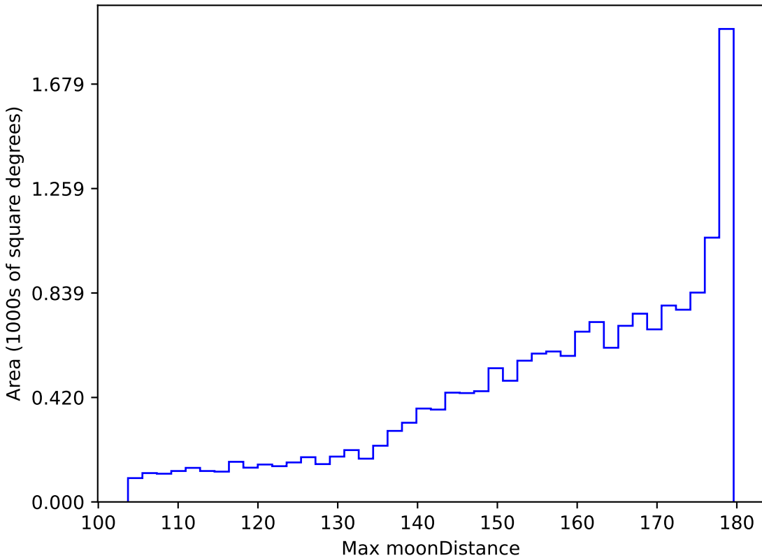
baseline_v2.1_10yrs WFD all bands: Max moonDistance
