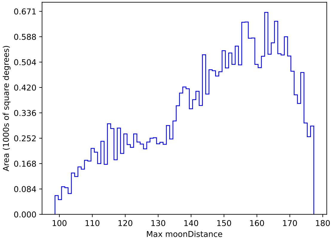
baseline_v2.1_10yrs All sky z band: Max moonDistance
