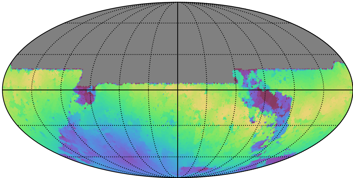
baseline_v2.1_10yrs All sky y band: Max moonDistance
