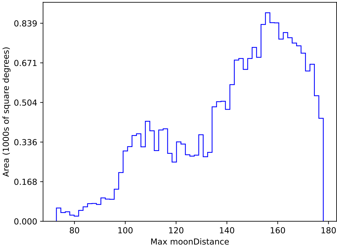
baseline_v2.1_10yrs All sky y band: Max moonDistance
