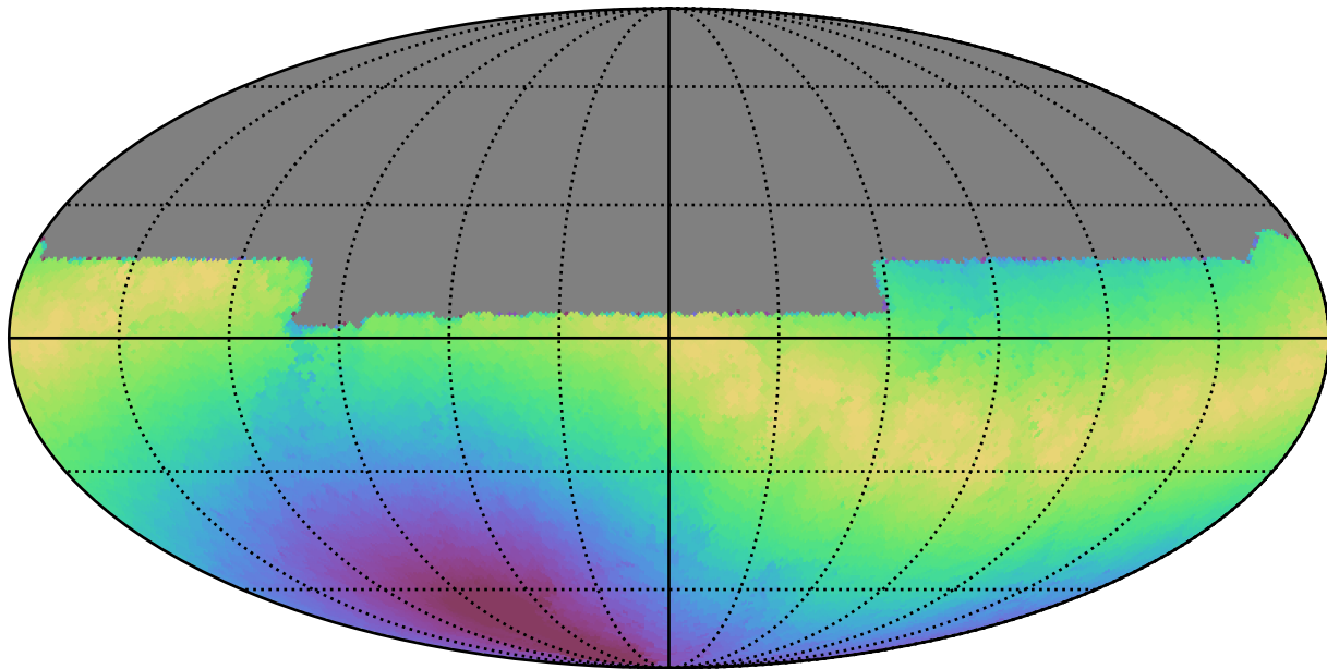
baseline_v2.1_10yrs All sky u band: Max moonDistance
