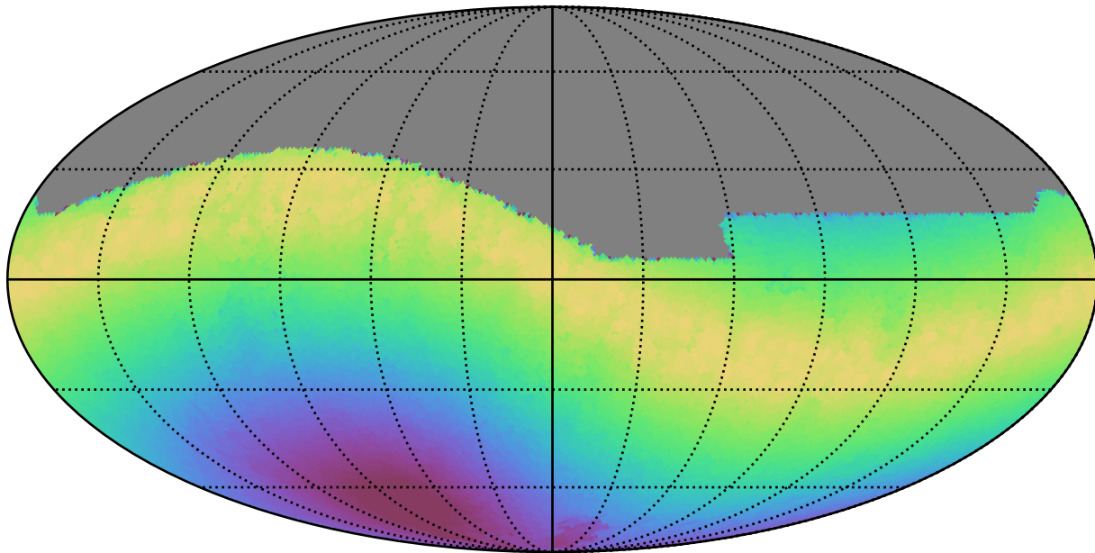
baseline_v2.1_10yrs All sky r band: Max moonDistance
