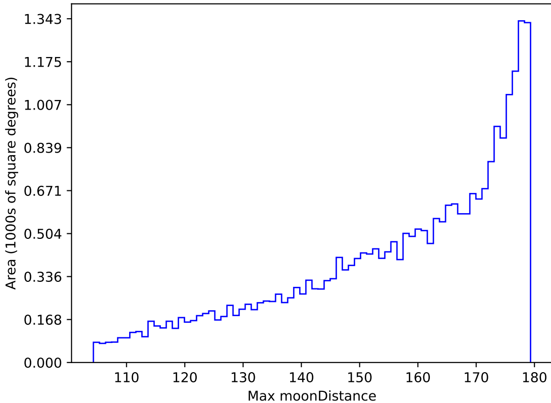
baseline_v2.1_10yrs All sky r band: Max moonDistance
