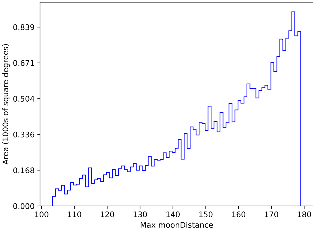
baseline_v2.1_10yrs All sky i band: Max moonDistance
