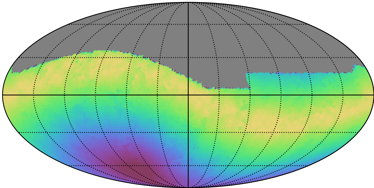
baseline_v2.1_10yrs All sky g band: Max moonDistance
